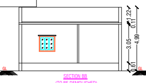
SECTION 88 (TO BE DEMOLISHED)
