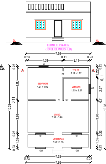
EXG. GROUND FLOOR PLAN (TO BE DEMOLISHED)
