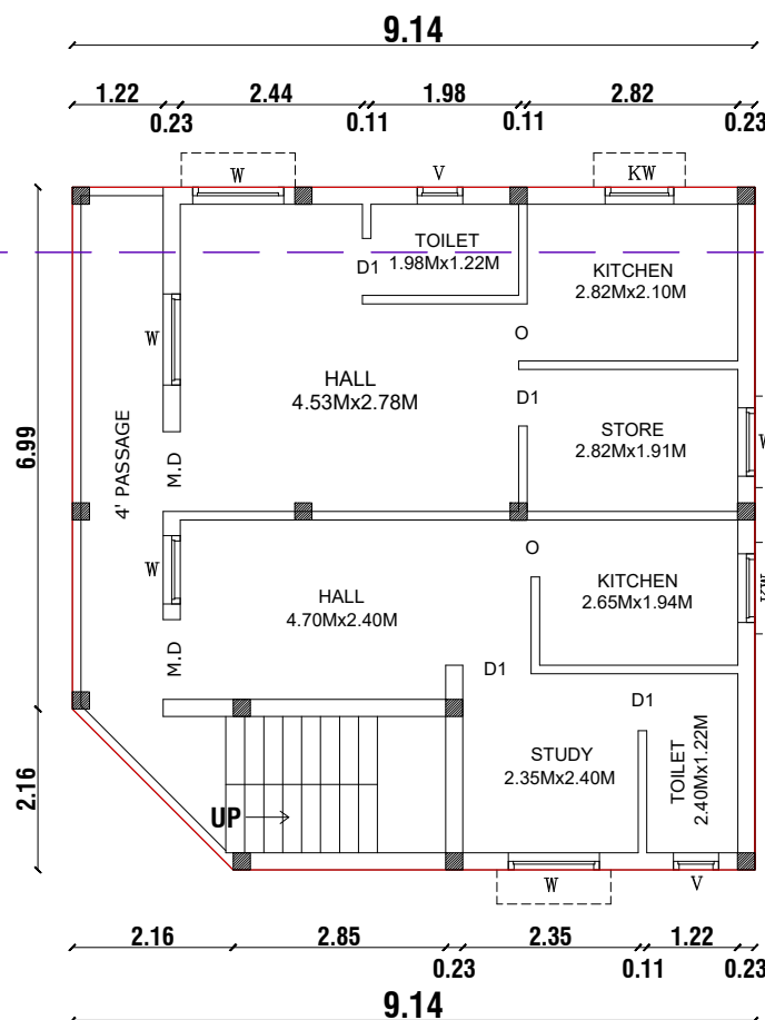
TYPICAL PRO.FIRST & PRO.SECOND FLOOR PLAN
