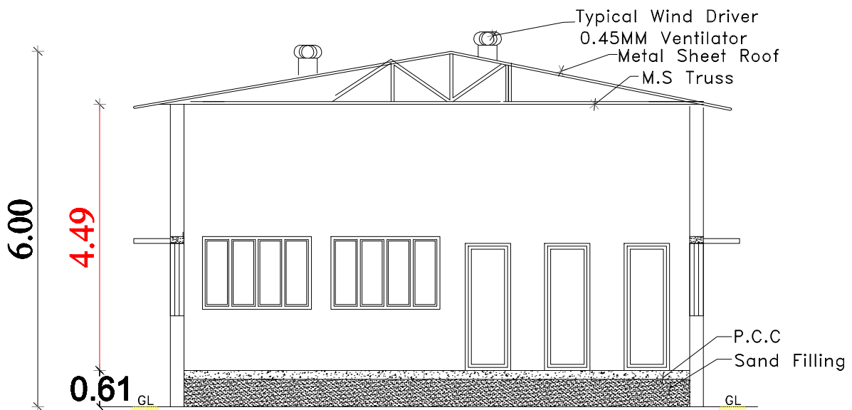
SECTION A-A PROPOSED
