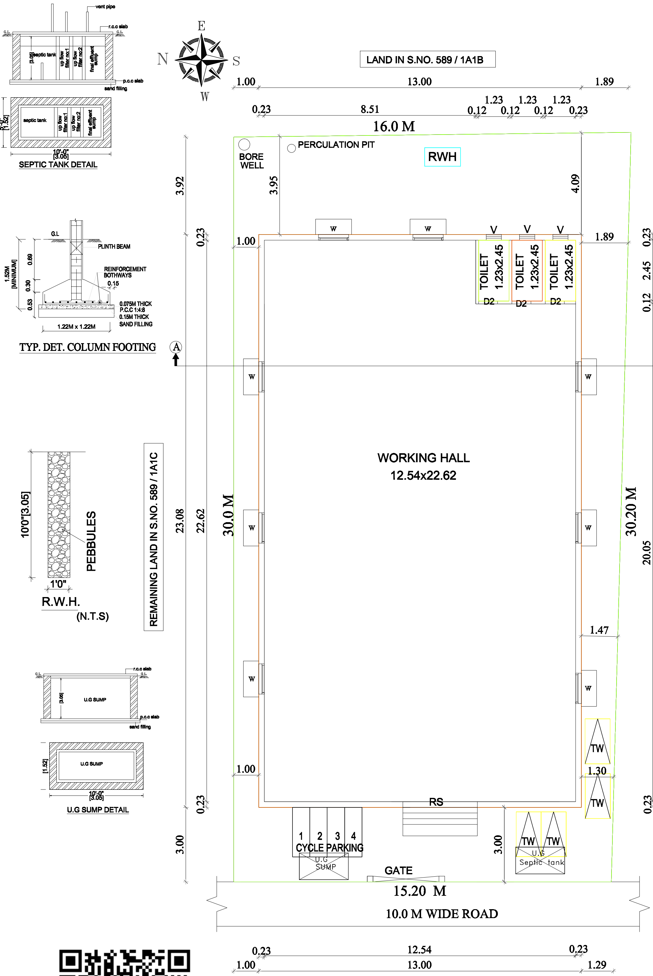
SITE CUM GROUND FLOOR PLAN PROPOSED
