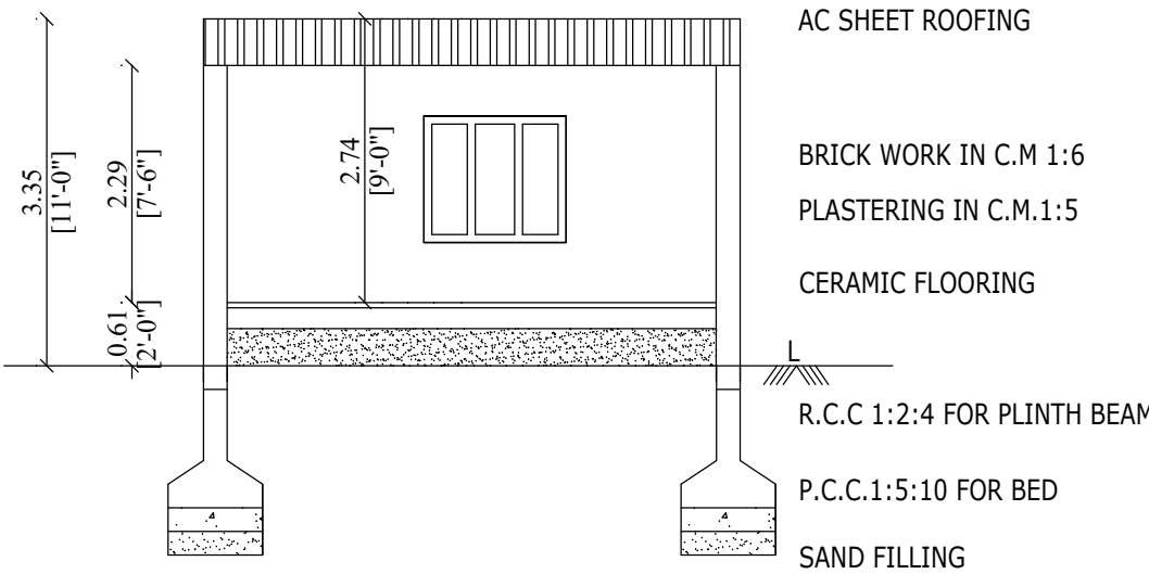
SECTION ON "LS"
