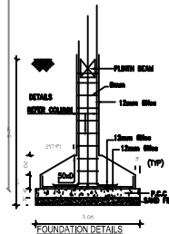
FOUNDATION DETAILS
