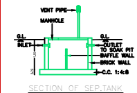
SECTION OF SEPTIC TANK
