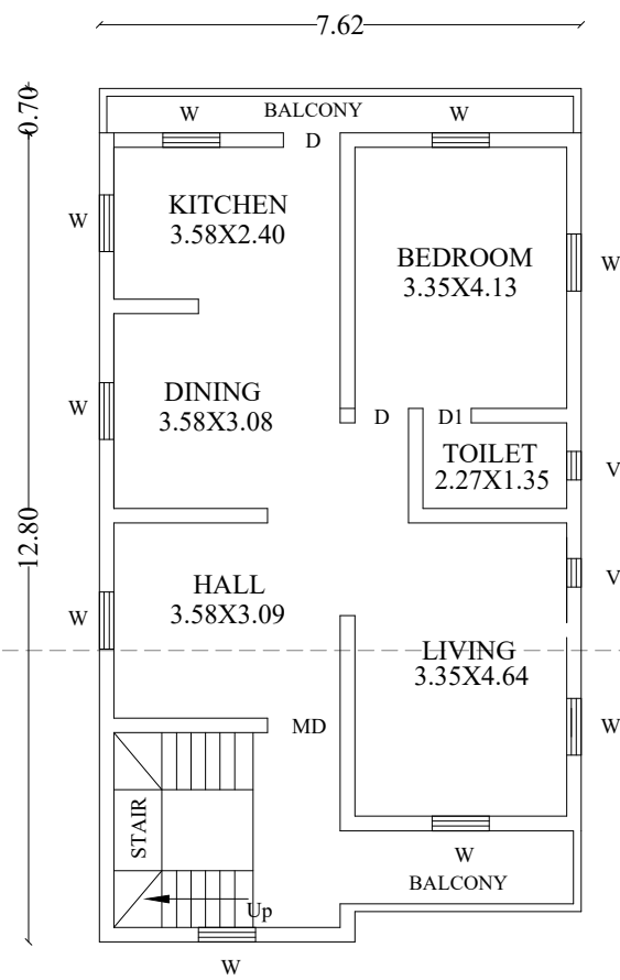
SECOND FLOOR
