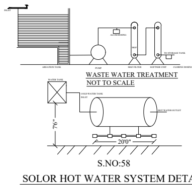
SOLOR HOT WATER SYSTEM DETAILS
