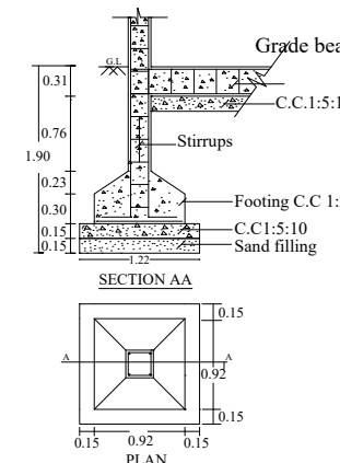
FOUNDATION DETAILS
