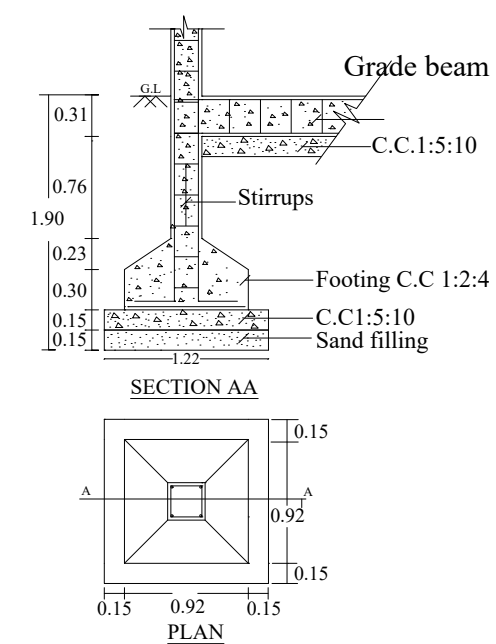
FOUNDATION DETAILS
