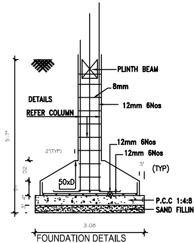
FOUNDATION DETAILS
