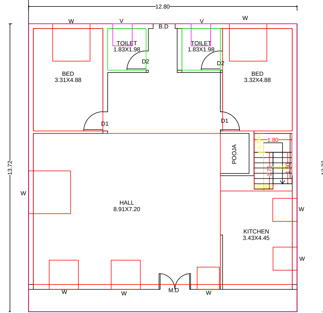
FLOOR PLAN
