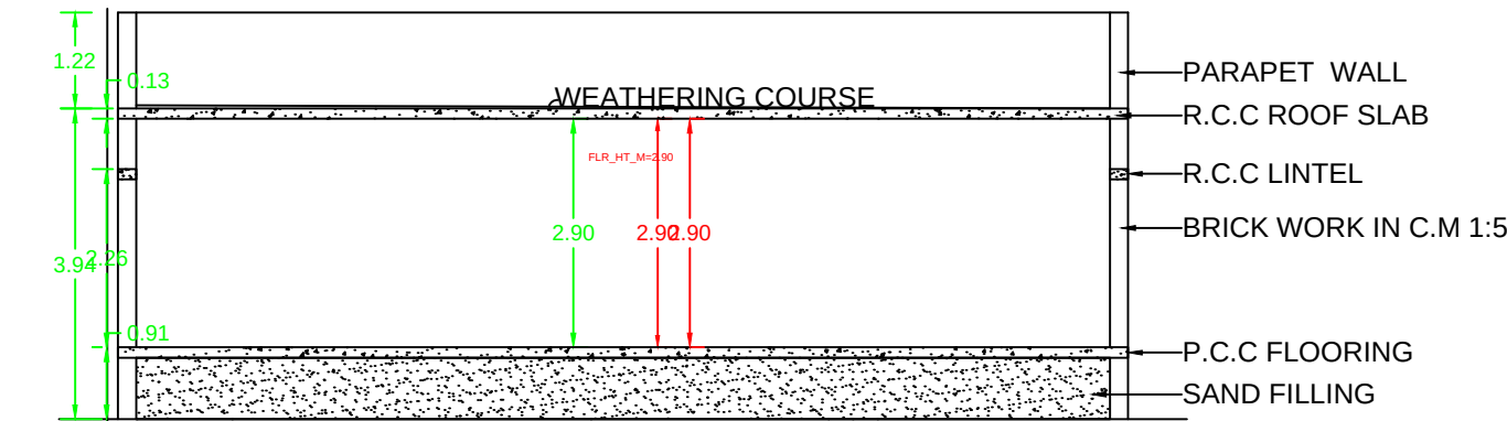
SECTION
