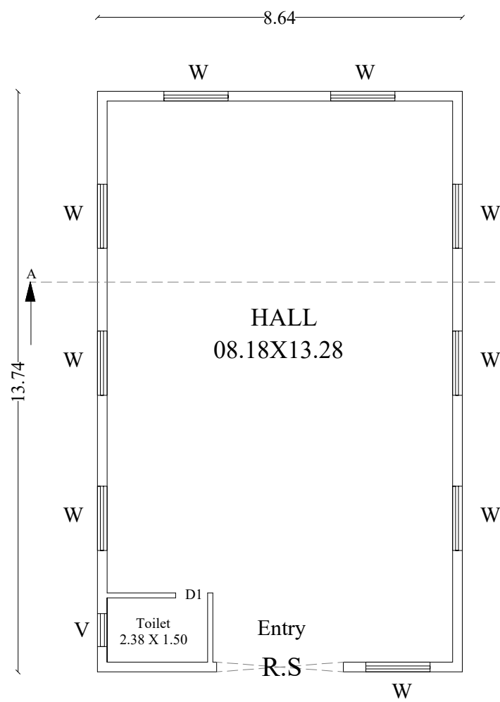
FLOOR
