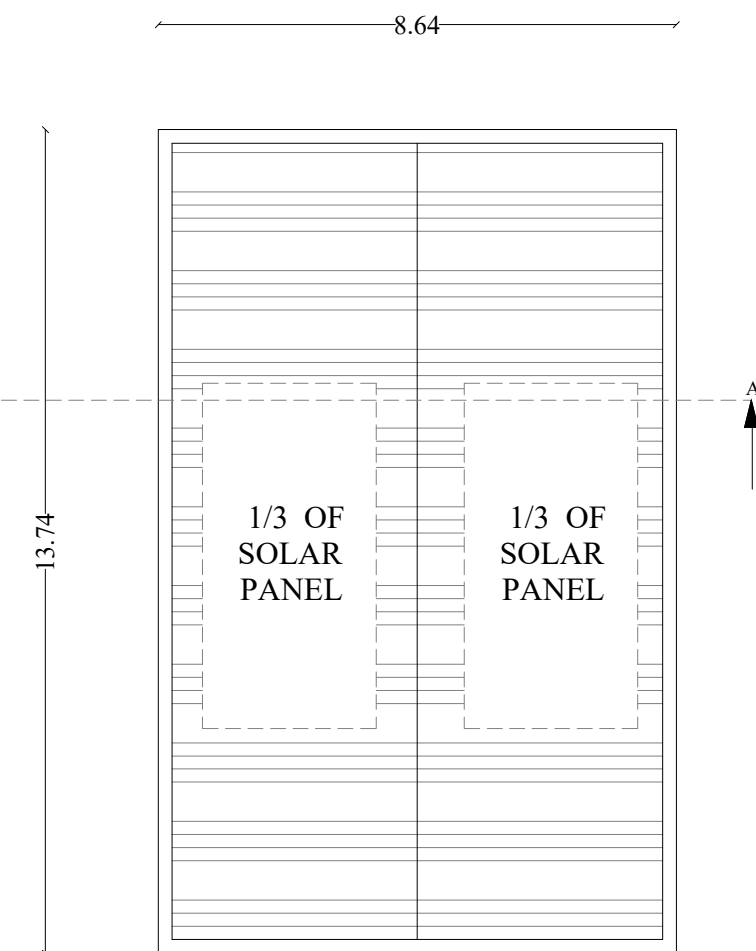
ROOF FLOOR
