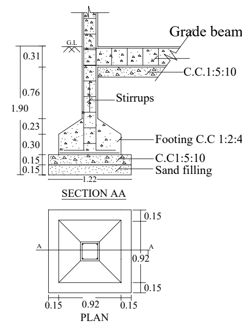
FOUNDATION DETAILS
