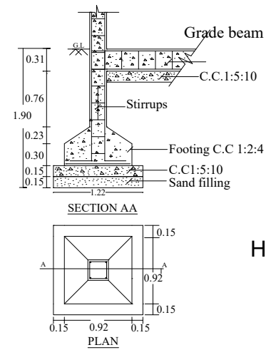
FOUNDATION DETAILS
