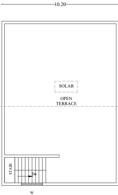
TERRACE FLOOR
