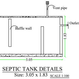
SEPTIC TANK DETAILS Size: 3.05 x 1.83 SCALE: 1:100
