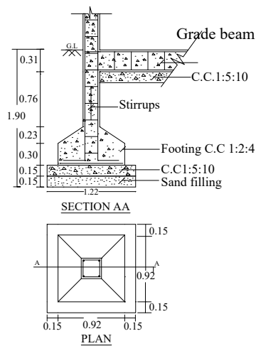
FOUNDATION DETAILS
