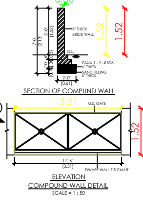
SECTION OF COMPOUND WALL
