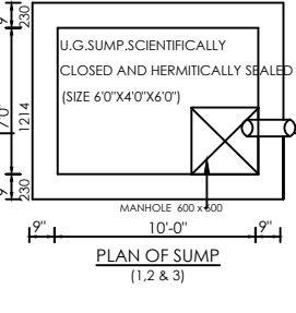
PLAN OF SUMP
