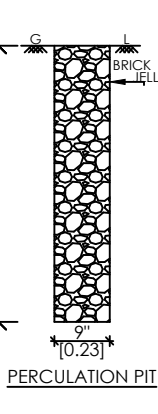
PERCOLATION PIT
