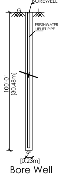
Bore Well
