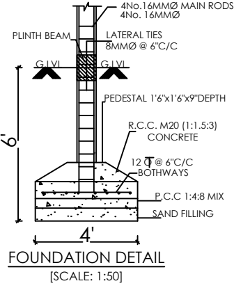
FOUNDATION DETAIL
