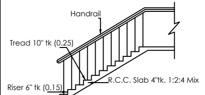
STAIRCASE DETAILS
