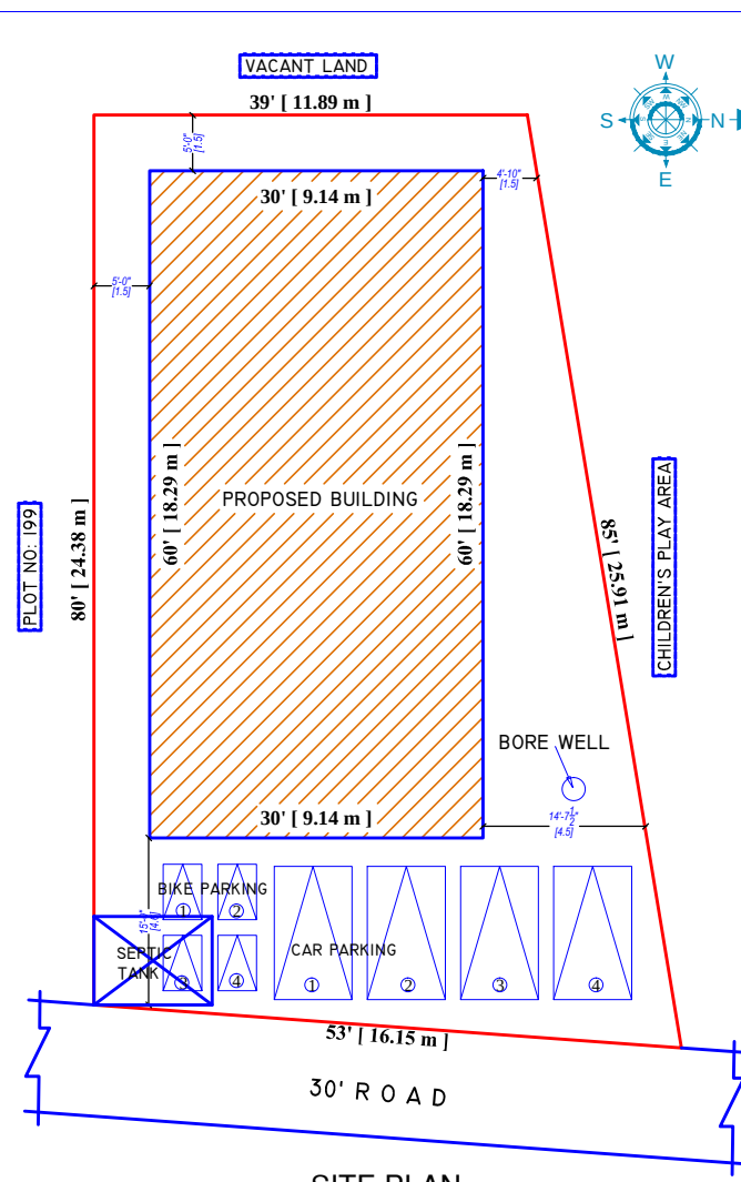
SITE PLAN
