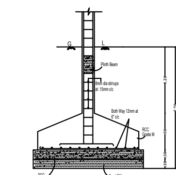
SECTION OF FOOTING
