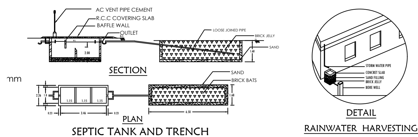
SEPTIC TANK AND TRENCH
