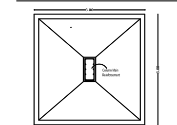
COLUMN FOUNDATION DETAIL PLAN OF FOOTING
