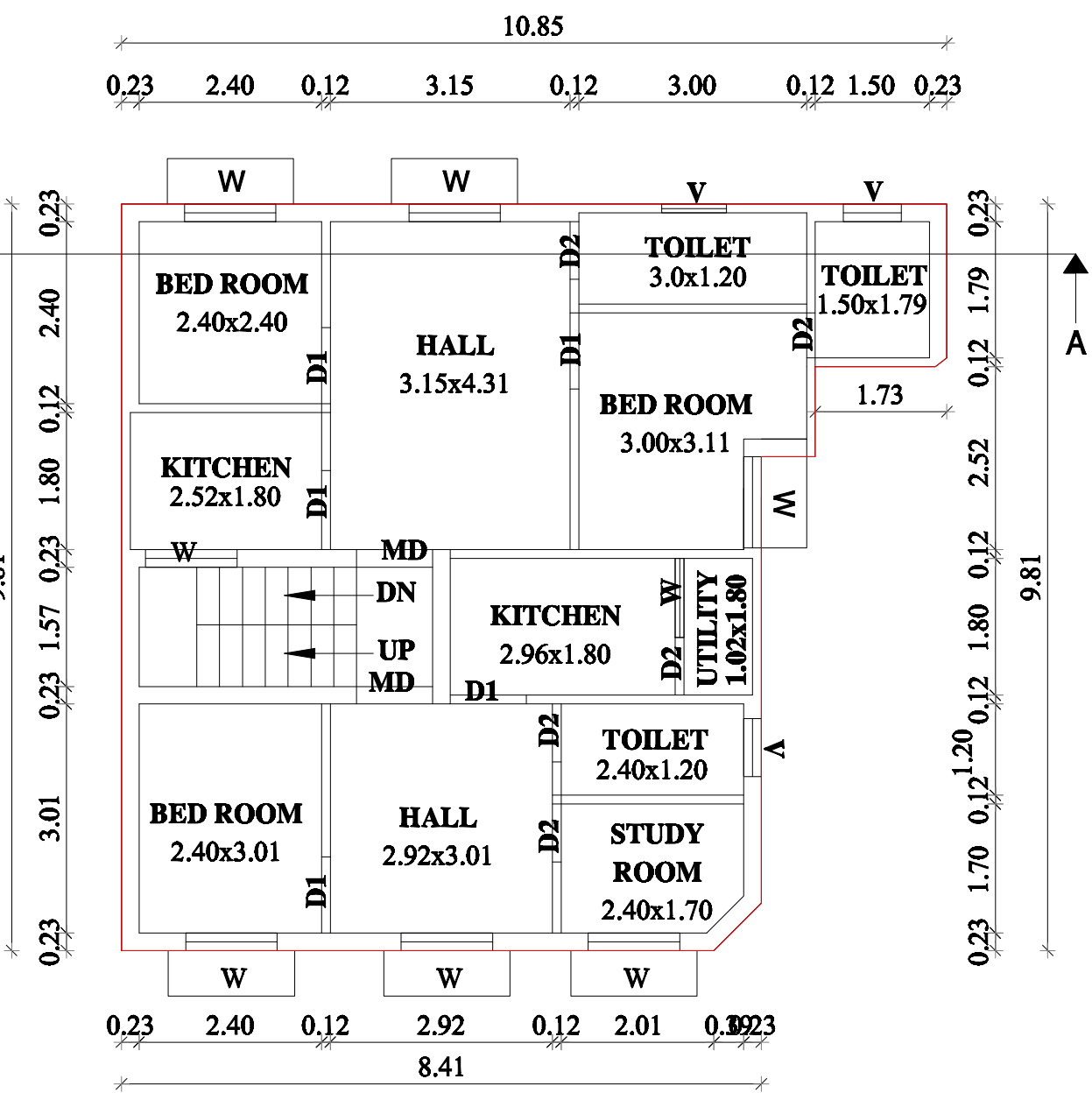
SECOND FLOOR PLAN PROPOSED
