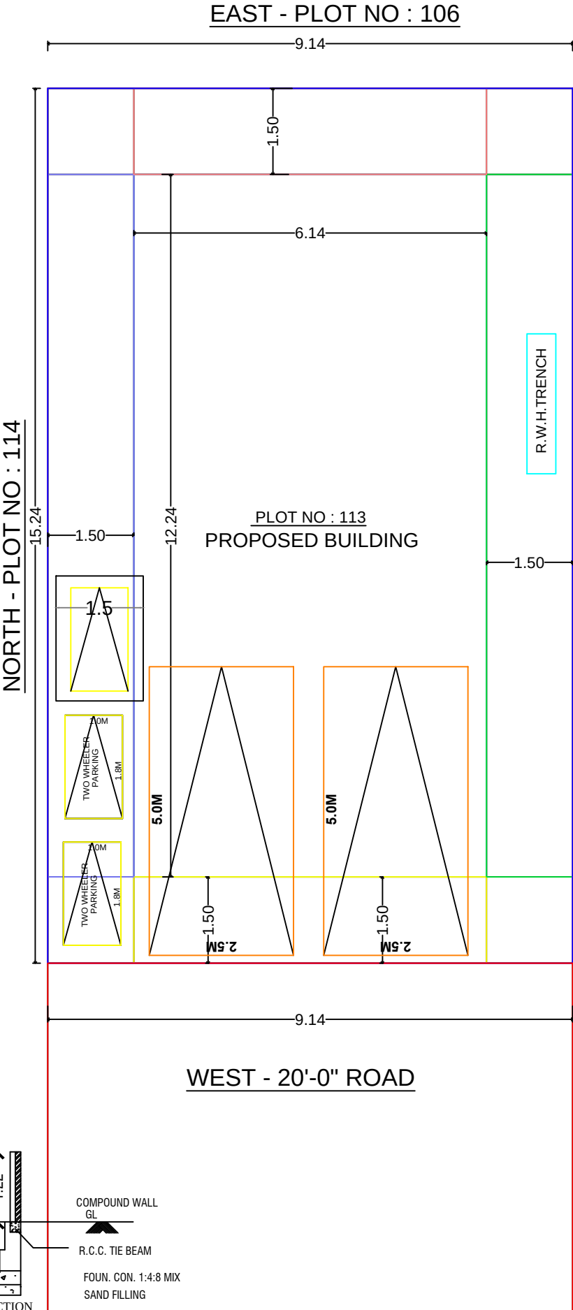
SITE PLAN
