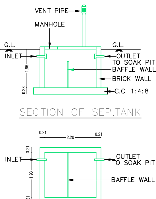
PLAN SEPTIC TANK
