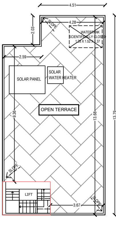
PROPOSED TERRACE PLAN
