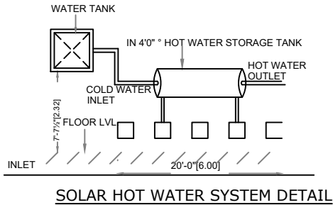
SOLAR HOT WATER SYSTEM DETAIL
