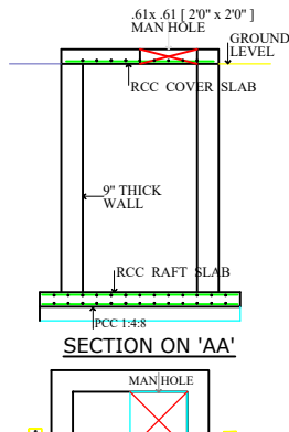
FOUNDATION DETAILS SCALE : 1:50
