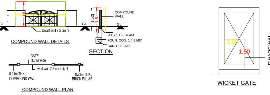
WICKET GATE
