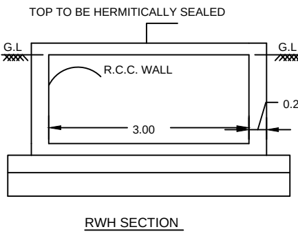
RWH SECTION
