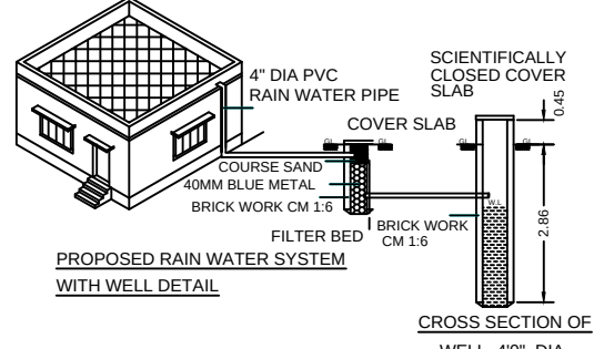
CROSS SECTION OF WELL 4' DIA
