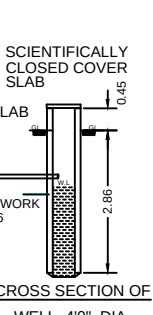
CROSS SECTION OF WELL 4' DIA
