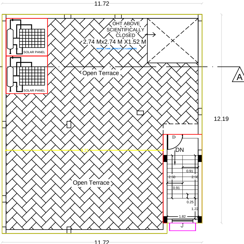
TERRACE PLAN
