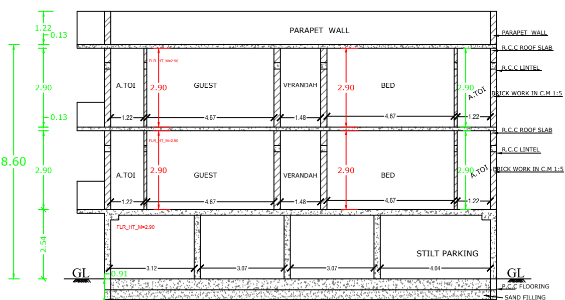
SECTION ON "IM"
