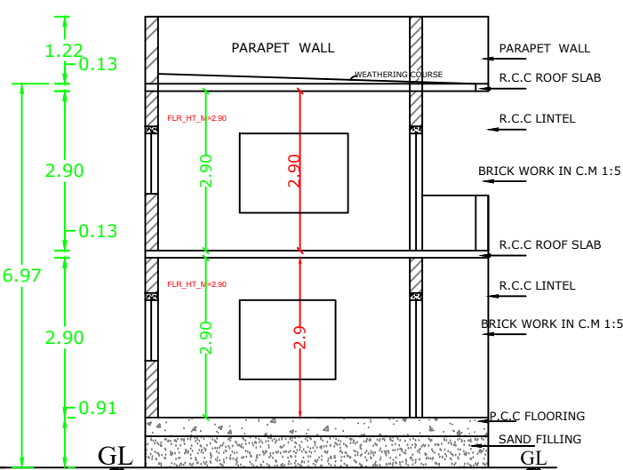
SECTION ON "IM"
