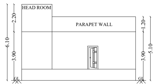
EAST FACING ELEVATION
