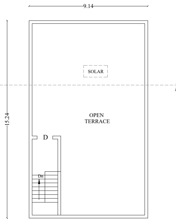
TERRACE FLOOR
