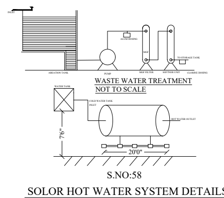
SOLOR HOT WATER SYSTEM DETAILS
