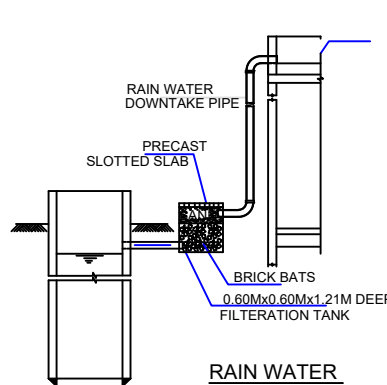
RAIN WATER
