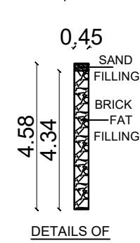
DETAILS OF PERCOLATION PIT
