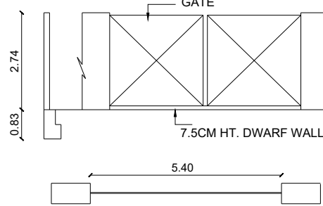
COMPOUND WALL WITH GATE
