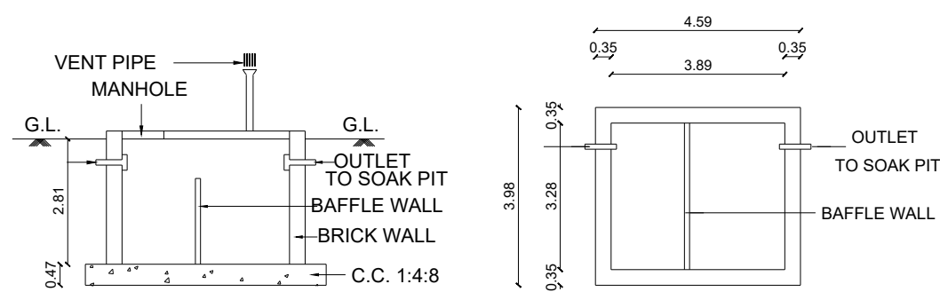
SECTION OF SEP.TANK
