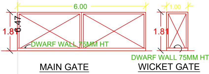
MAIN GATE
