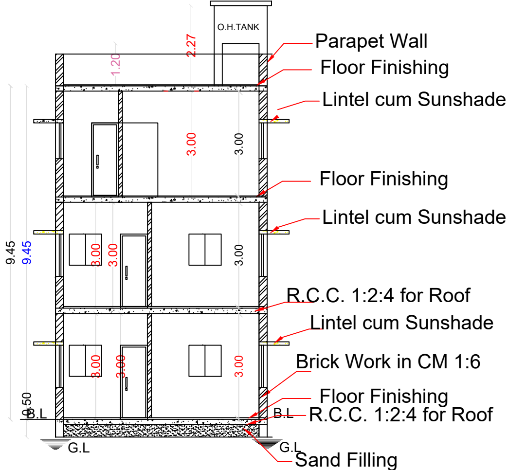
CROSS SECTION ON "AB"
