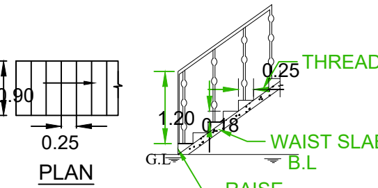
STAIRCASE DETAILS
