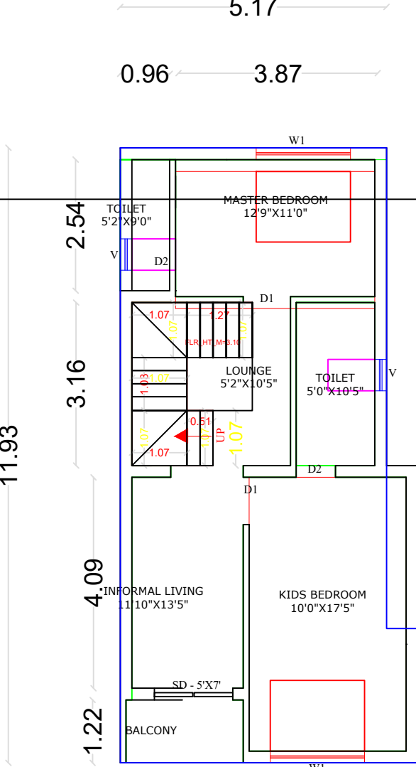
SF FLOOR PLAN
