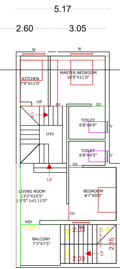
FF FLOOR PLAN
