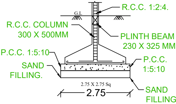
FOUNDATION DETAIL
