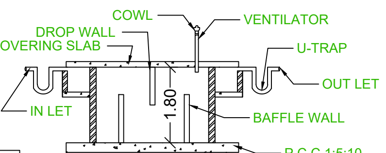
SECTION ON 'XY' SEPTIC TANK DETAILS PLAN
