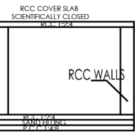
SECTION X-X
