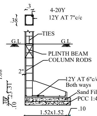
TYPICAL SECTION OF FOOTING
