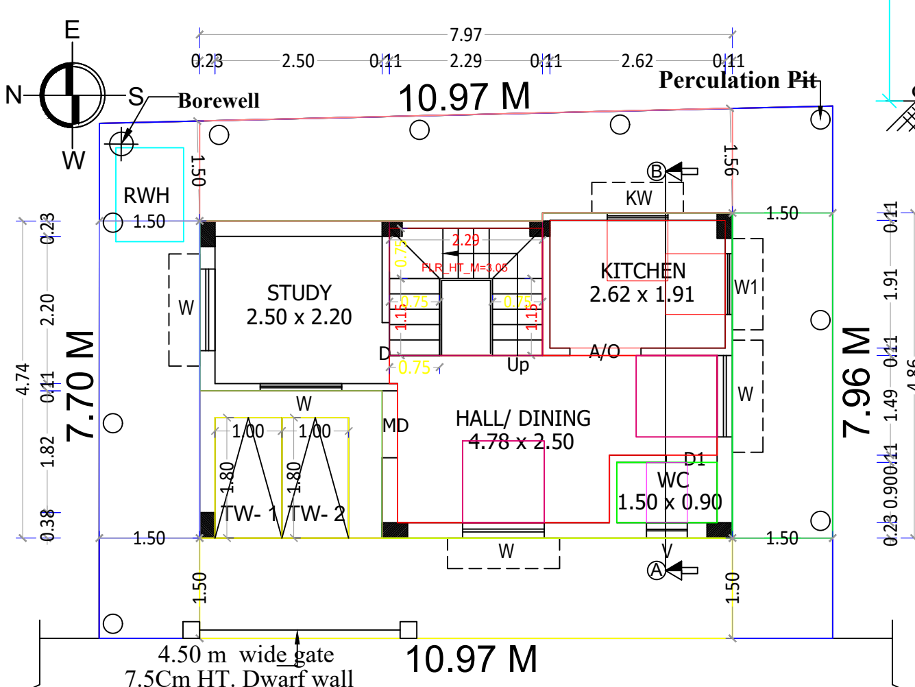
SITE CUM GROUND FLOOR PLAN (PROPOSED)
