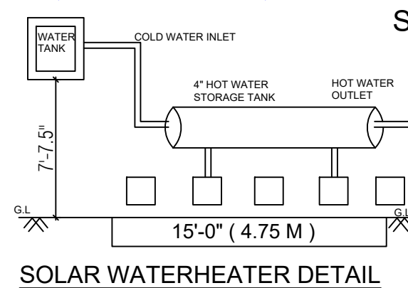
SOLAR WATERHEATER DETAIL
