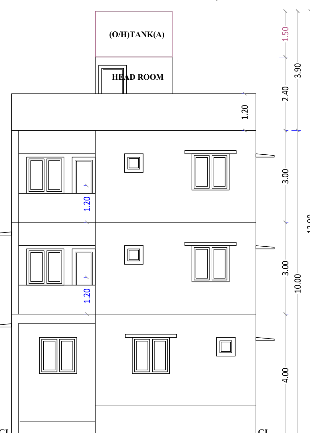
FRONT ELEVATION (PROPOSED)
