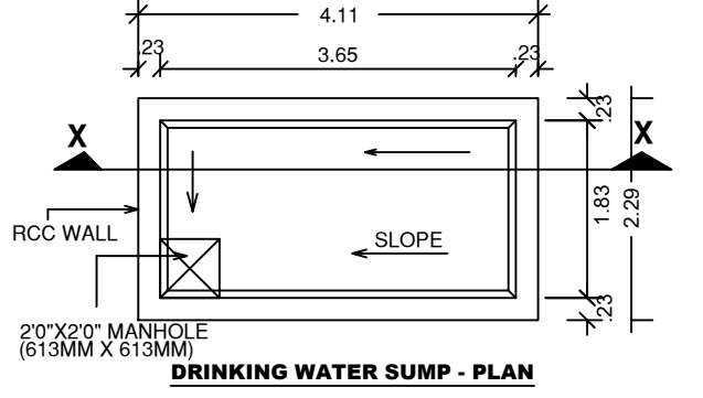
SUMP DETAIL
