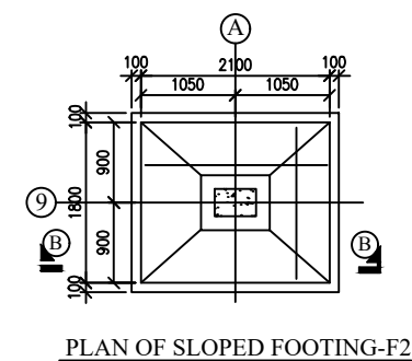
PLAN OF SLOPED FOOTING-F2
