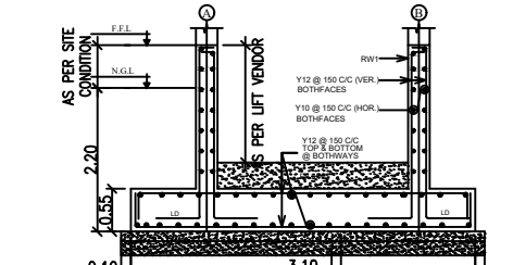
PLAN OF COMBINED FOOTING
