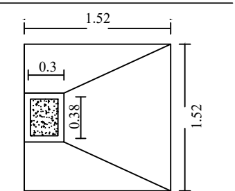
PLAN OF FOUNDATION
