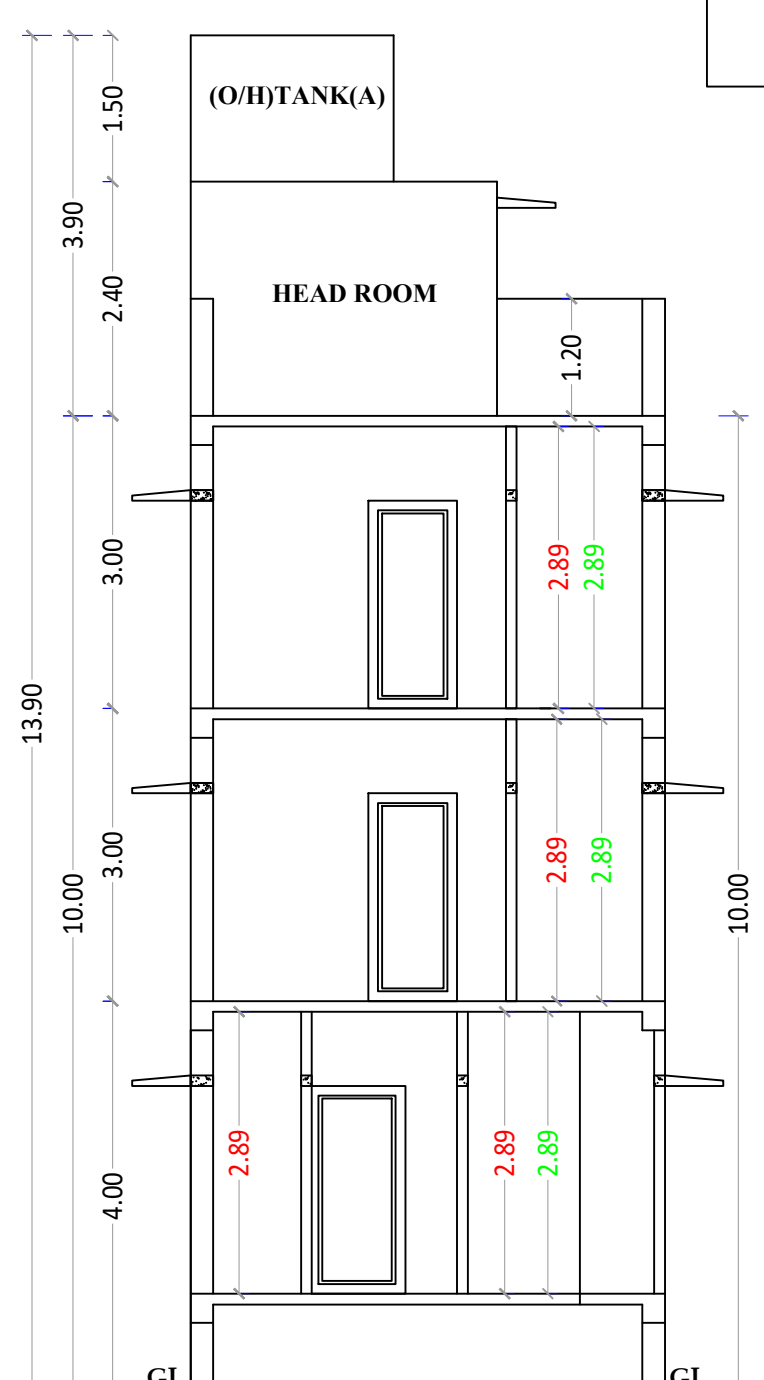
SECTION ON 'A-A' (PROPOSED)
