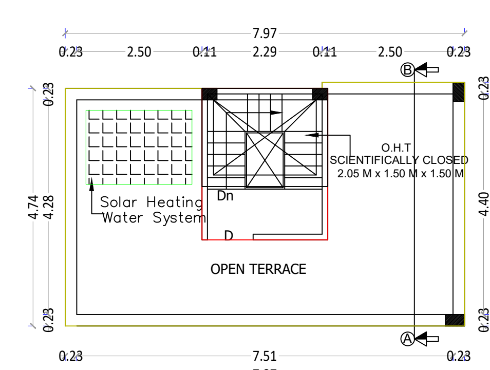
TERRACE FLOOR PLAN (PROPOSED)
