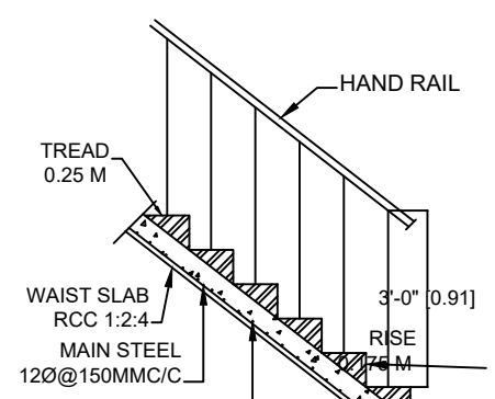
STAIRCASE DETAIL
