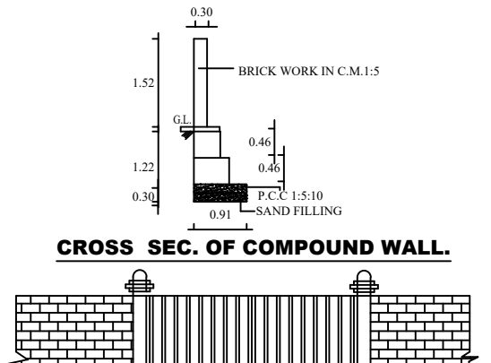
CROSS SEC. OF COMPOUND WALL
