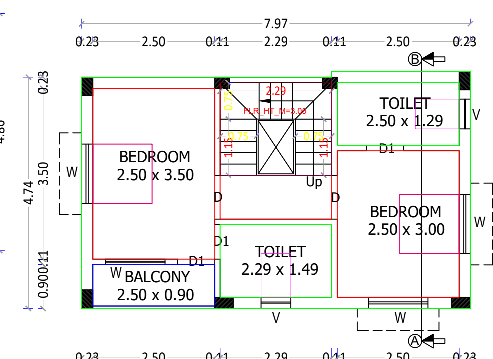
FIRST FLOOR PLAN (PROPOSED)
