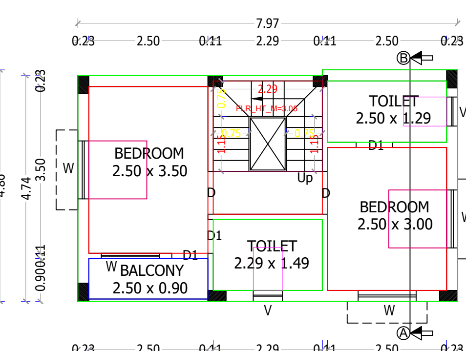
SECOND FLOOR PLAN (PROPOSED)
