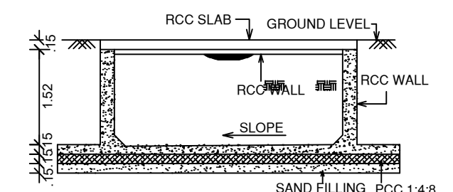
SECTION AT 'XX'
