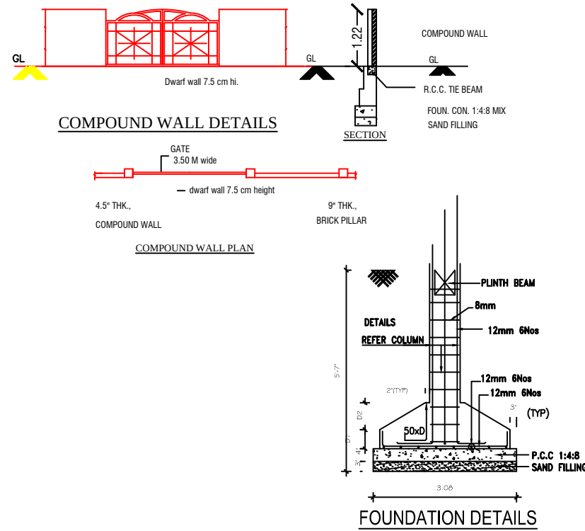
FOUNDATION DETAILS
