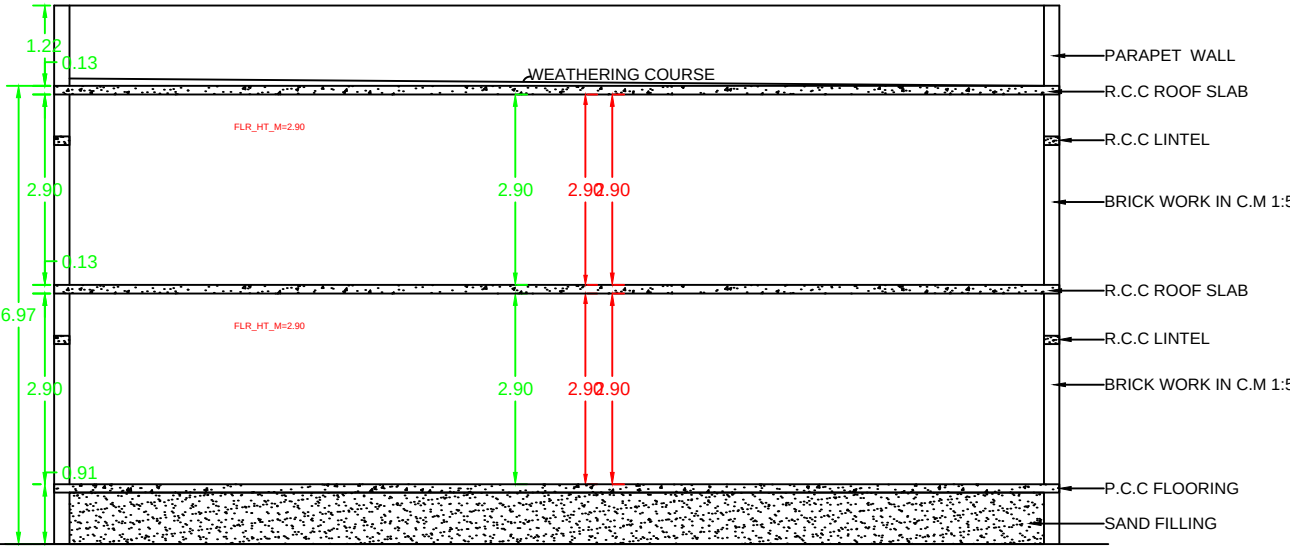
SECTION
