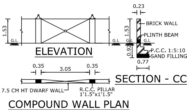
COMPOUND WALL PLAN
