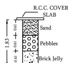
SECTION
