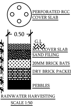
RAINWATER HARVESTING SCALE 1:50
