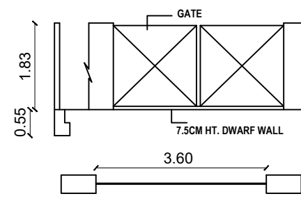
COMPOUND WALL WITH DWARF WALL DETAILS
