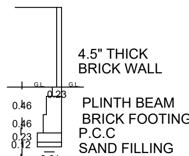
COMPOUND WALL
