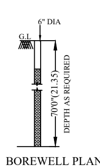
BOREWELL PLAN
