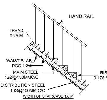
STAIR CASE DETAILS SCALE 1:300
