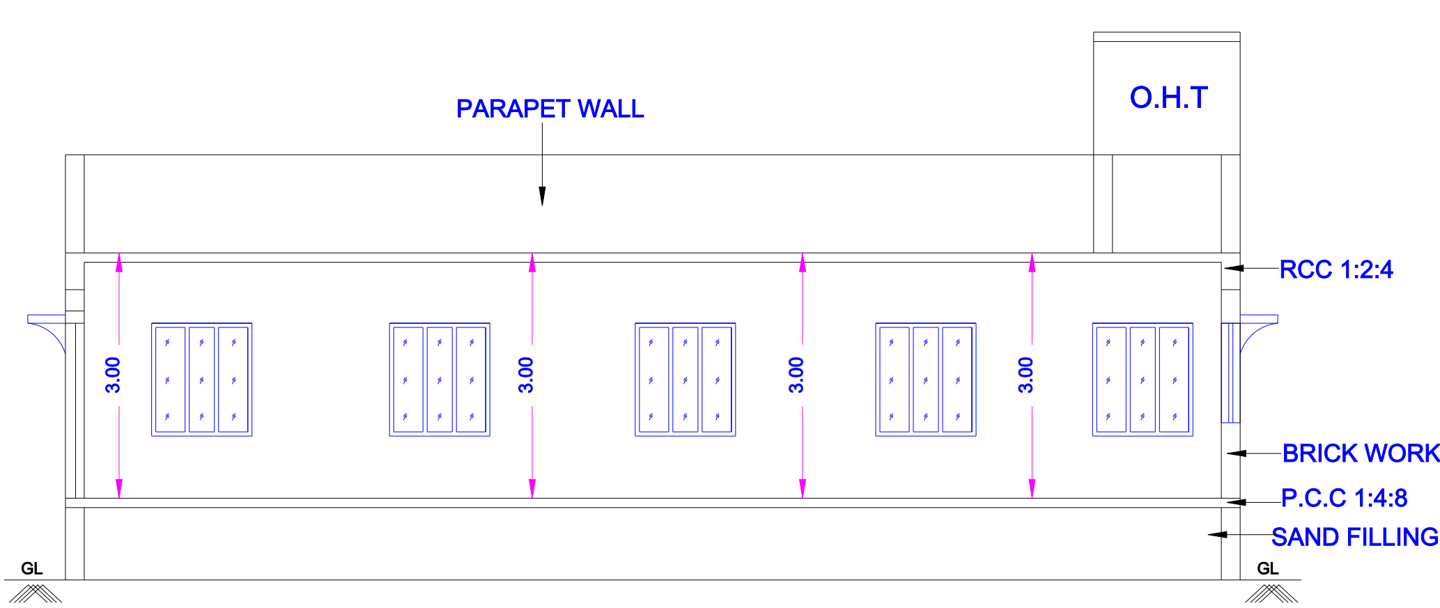
CROSS SECTION - AB (PROPOSED)
