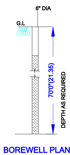
BOREWELL PLAN
