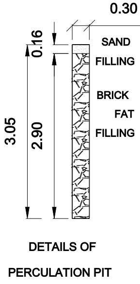
DETAILS OF PERCOLATION PIT
