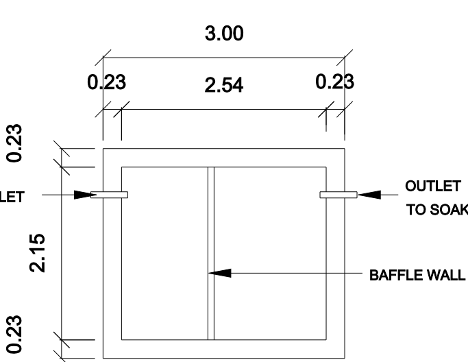
PLAN SEPTIC. TANK
