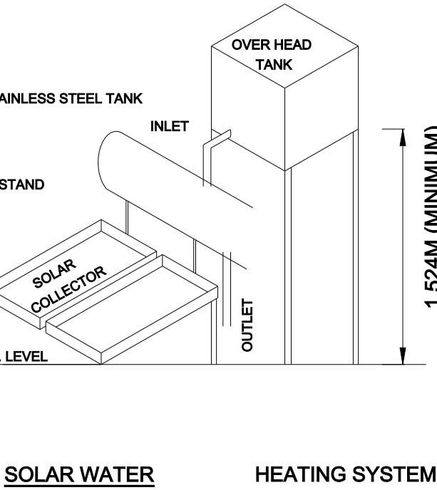
SOLAR WATER HEATING SYSTEM
