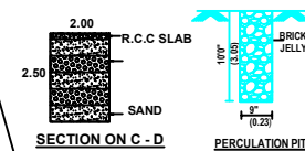
SECTION ON C - D
