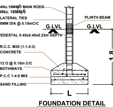
FOUNDATION DETAIL [SCALE: 1:50]
