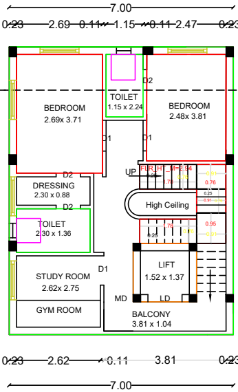
PRO.SECOND FLOOR PLAN
