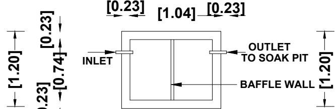
PLAN SEPTIC. TANK
