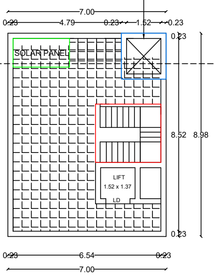
PRO.TERRACE FLOOR PLAN
