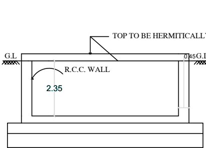
RWK SECTION (SAMPLE) RWK_CAPACITY_L=2000LTRS
