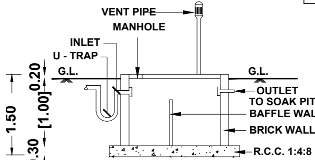
SECTION OF SEP.TANK
