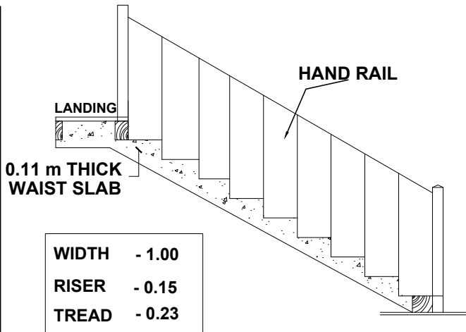
STAIRCASE DETAIL
