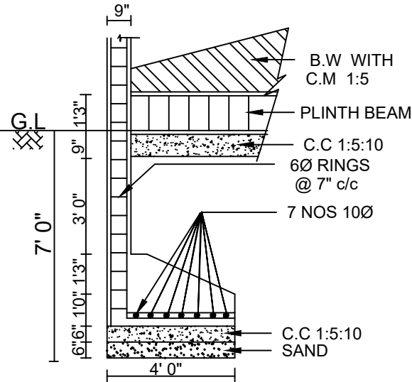
FOUNDATION DETAILS SCALE : 1/4 INCHES TO A FOOT
