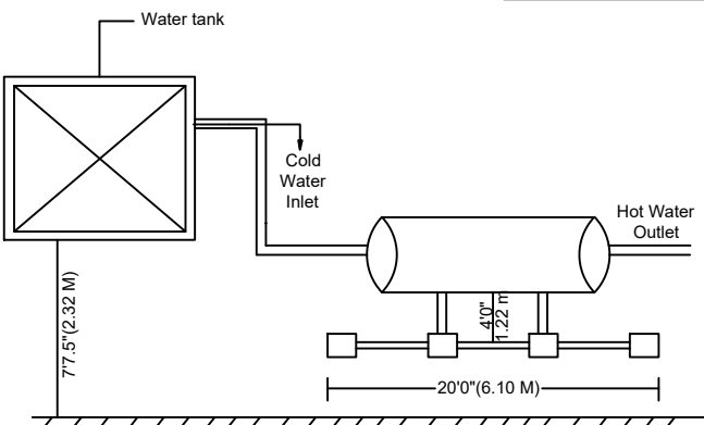
SOLAR ACTIVATION PLAN
