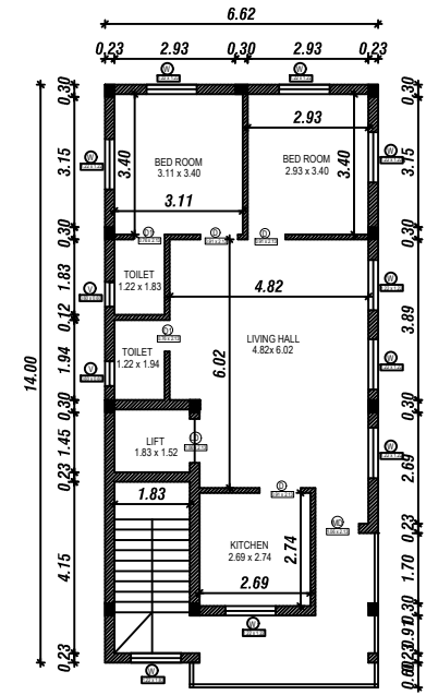
PROP. FIRST FLOOR PLAN
