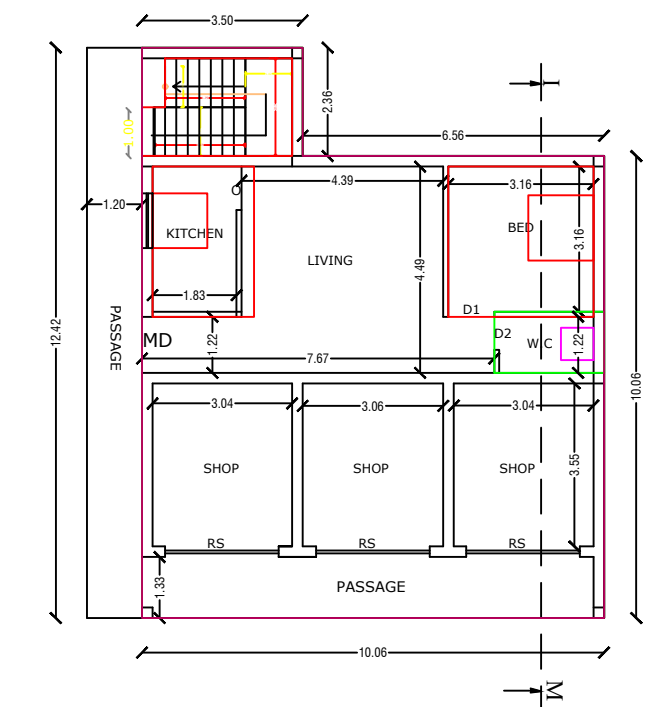
EXISTING APPROVED GROUND FLOOR PLAN
