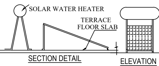
SECTION DETAIL
