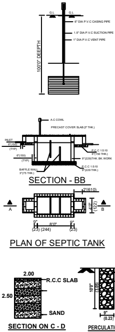
SECTION ON C - D
