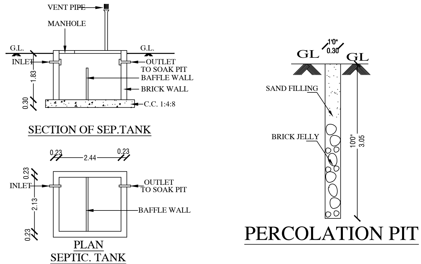
PLAN SEPTIC TANK
