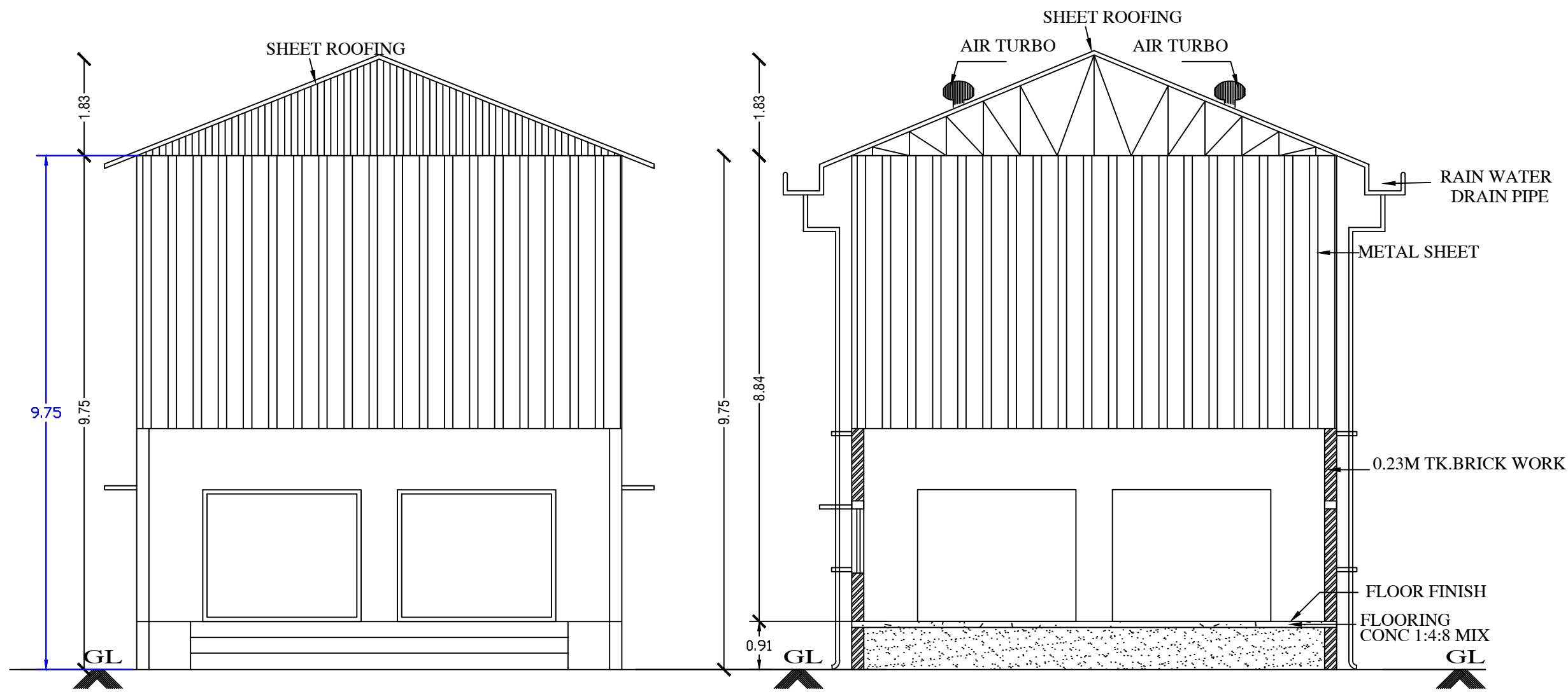
FRONT ELEVATION
