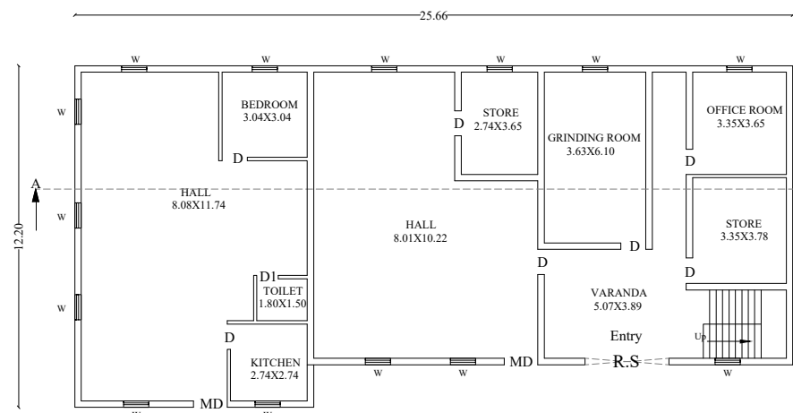
NORTH FACING EXISTING COMMERCIAL & ADDITIONAL RESIDENTIAL GROUND FLOOR
