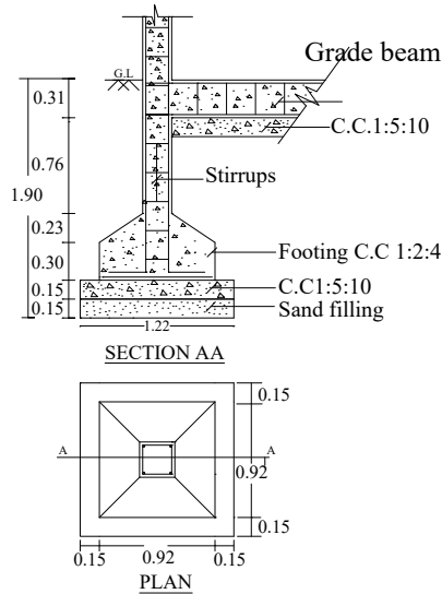
FOUNDATION DETAILS
