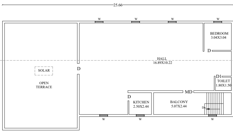
PROPOSED RESIDENTIAL SECOND FLOOR
