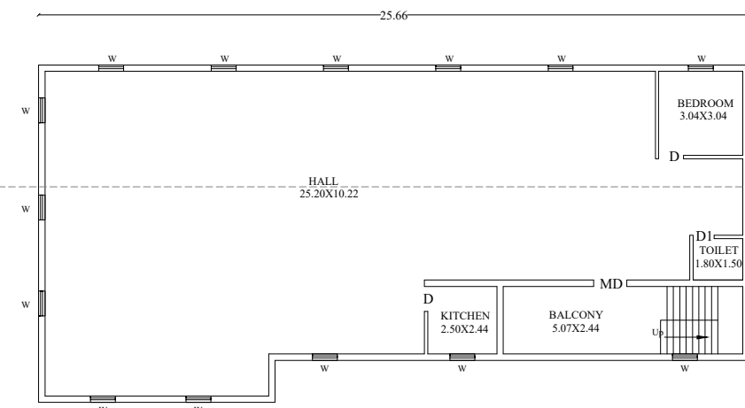
PROPOSED RESIDENTIAL FIRST FLOOR
