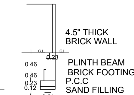
COMPOUND WALL
