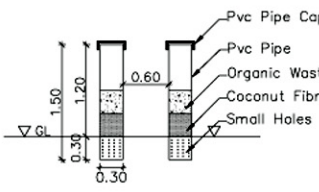
PIPE COMPOST PIT
