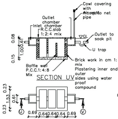
SEPTIC TANK PLAN
