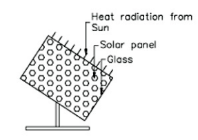
SOLAR SYSTEM
