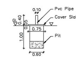
SOLID WASTE COMPOST PIT
