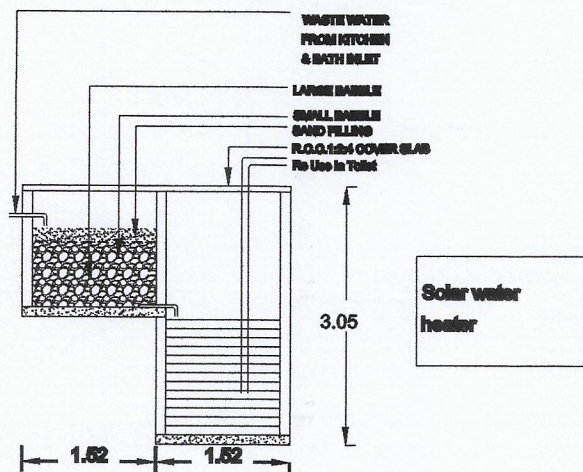
RECYCLING OF WASTE WATER FROM KITCHEN & BATHROOM
