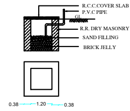
RAIN WATER HARVEST ARRANGEMENTS
