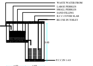
RECYCLING OF WASTE WATER FROM BATH
