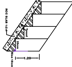
STAIR DETAILS
