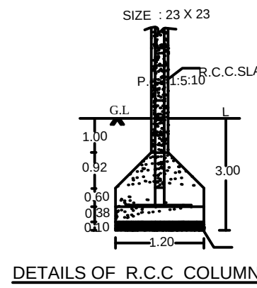
DETAILS OF R.C.C. COLUMN
