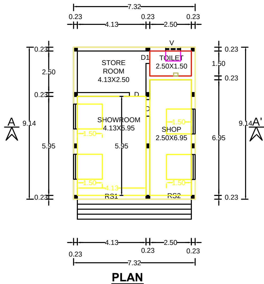
PLAN
