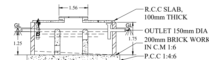
SECTION OF SEPTIC TANK
