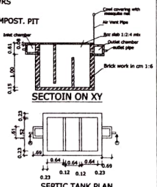
SEPTIC TANK PLAN
