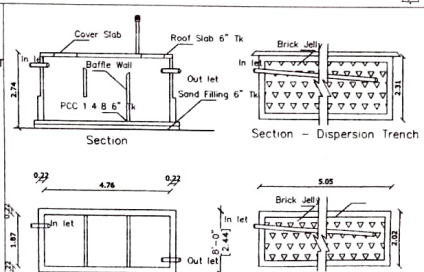
Plan - Septic Tank
